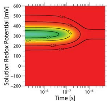
Fig. 9 Re-reduction kinetics of SP in dependence of the redox potential of the solution. The overall re-reduction kinetics of SP shown in (a) is a sum of the kinetic plots of the microstates in (b)–(f). The color and the contours indicate the oxidation probability of SP (blue—fully oxidized; red—fully reduced) or the probabilities of the microstates (blue—populated to 100%; red—unpopulated).
